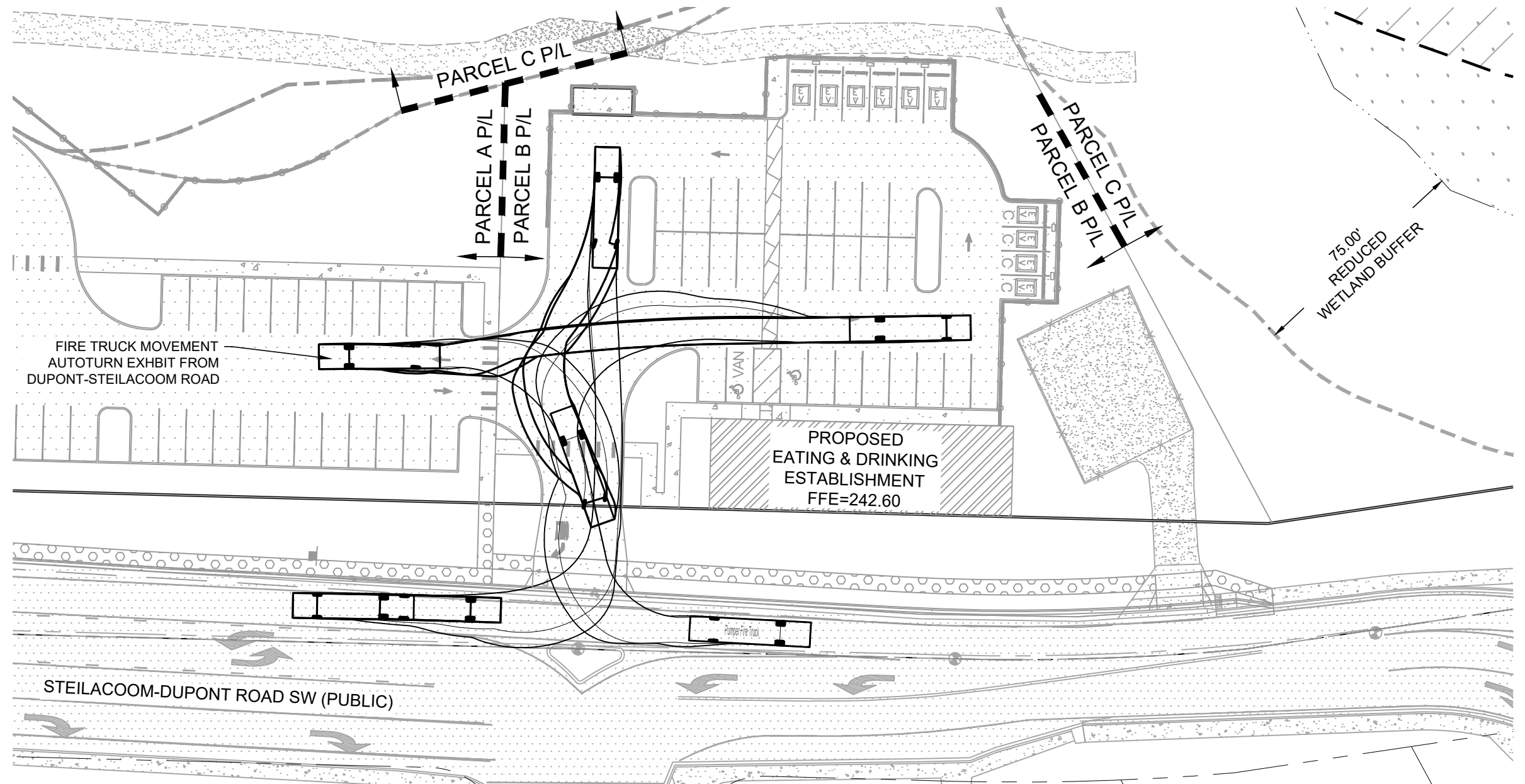
FIRE TRUCK TURNING MOVEMENT ACCESSING FROM STEILACOOM-DUPONT ROAD SW SCALE: 1" = 40'
