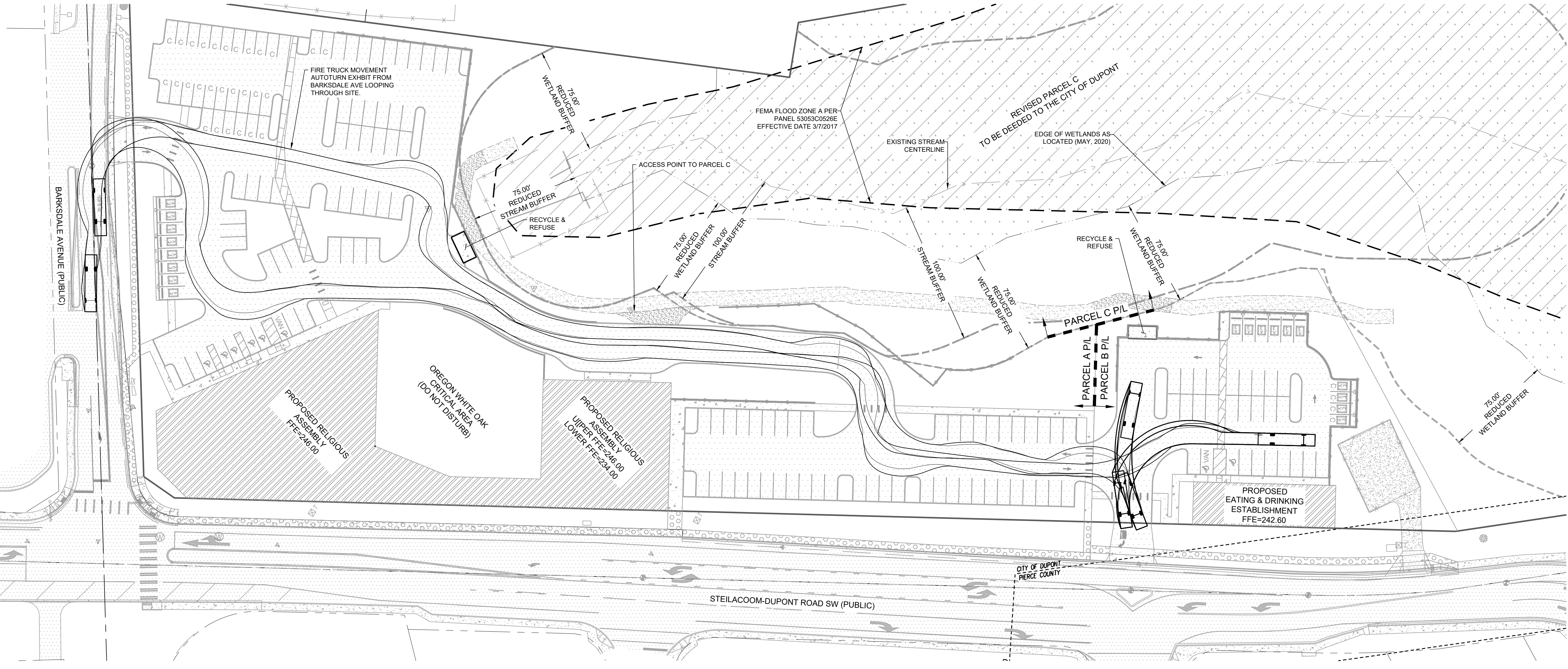
FIRE TRUCK TURNING MOVEMENT ACCESSING FROM BARKSDALE AVENUE. SCALE: 1" = 40'
