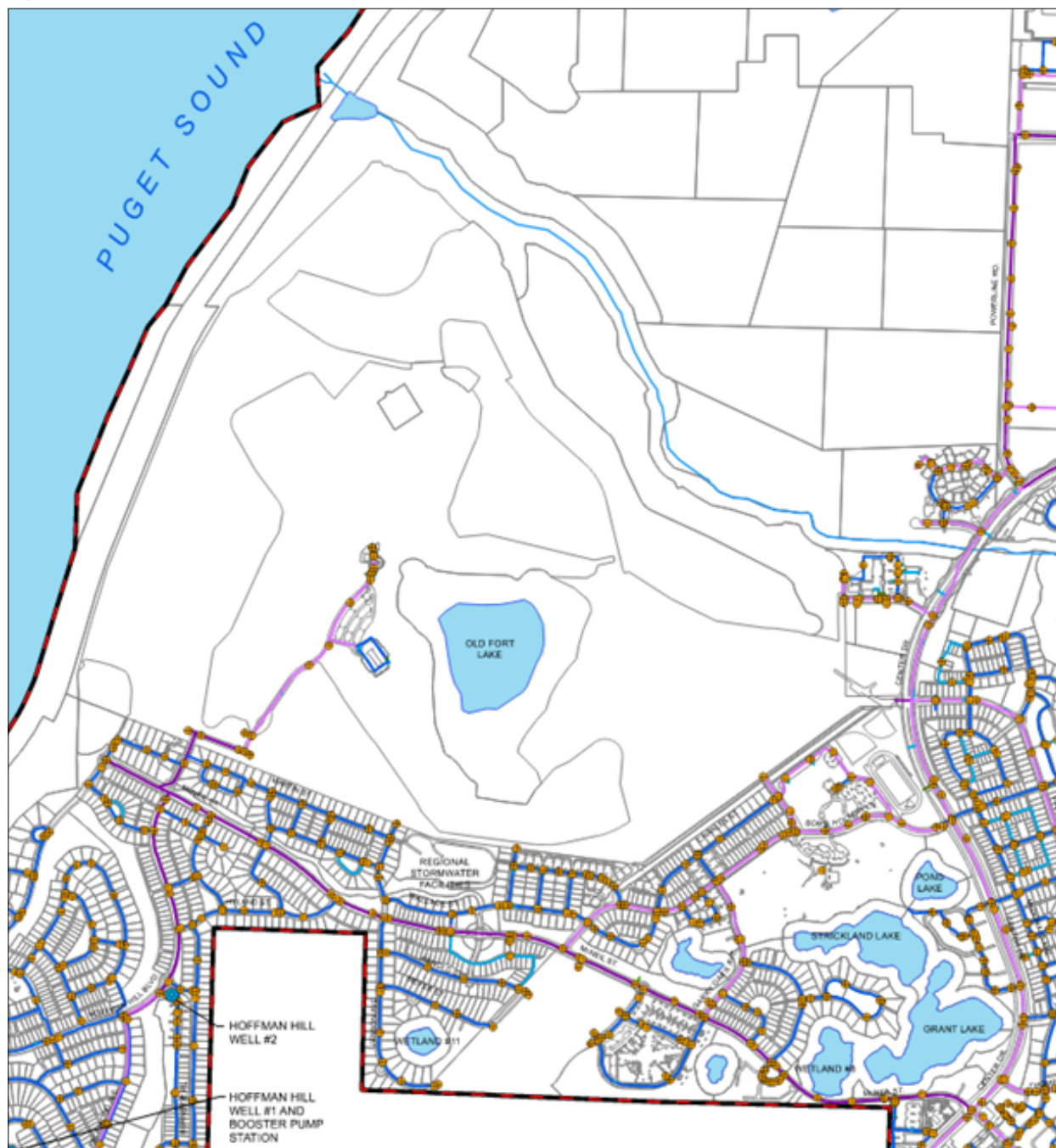
Figure 7-1. Water System Facilities Map
