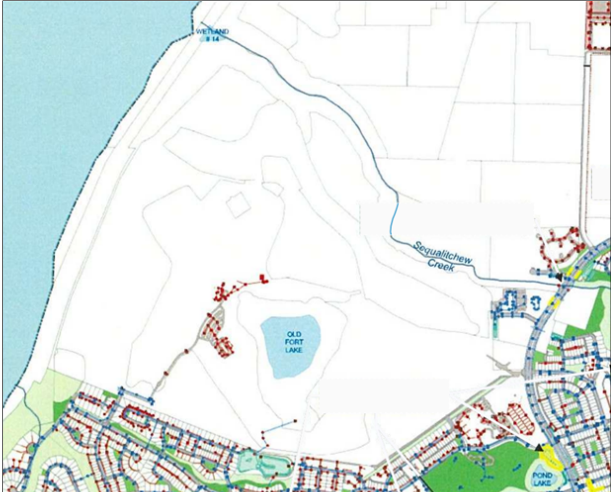
Figure 7-2. Sewer System Facilities Map
