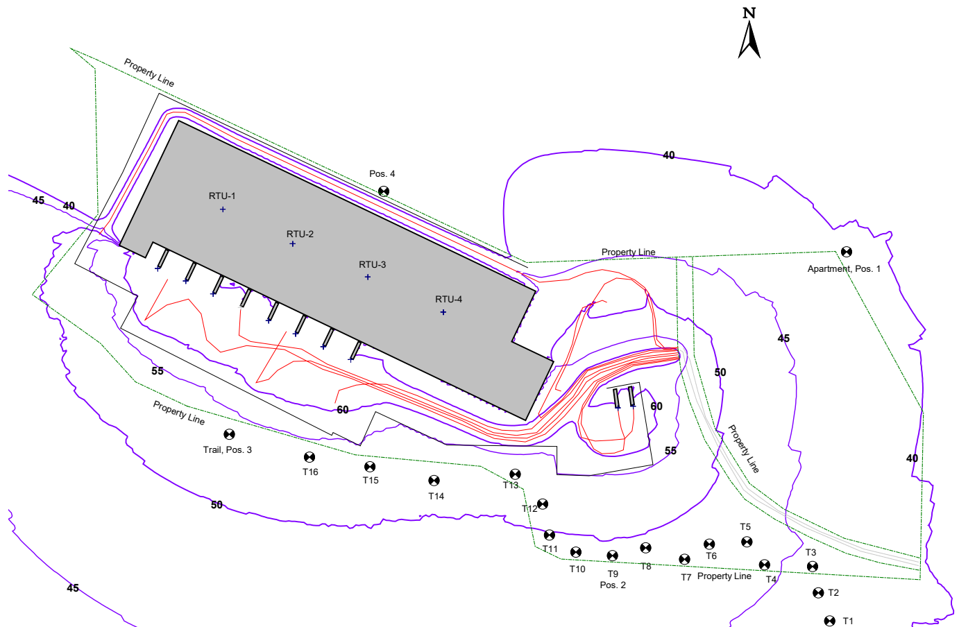
Figure 6. Noise level contours (dBA) and receiver locations for the 6 AM hour. Noise contours are evaluated at an elevation that is 5 feet above the pavement elevation at the loading docks.
