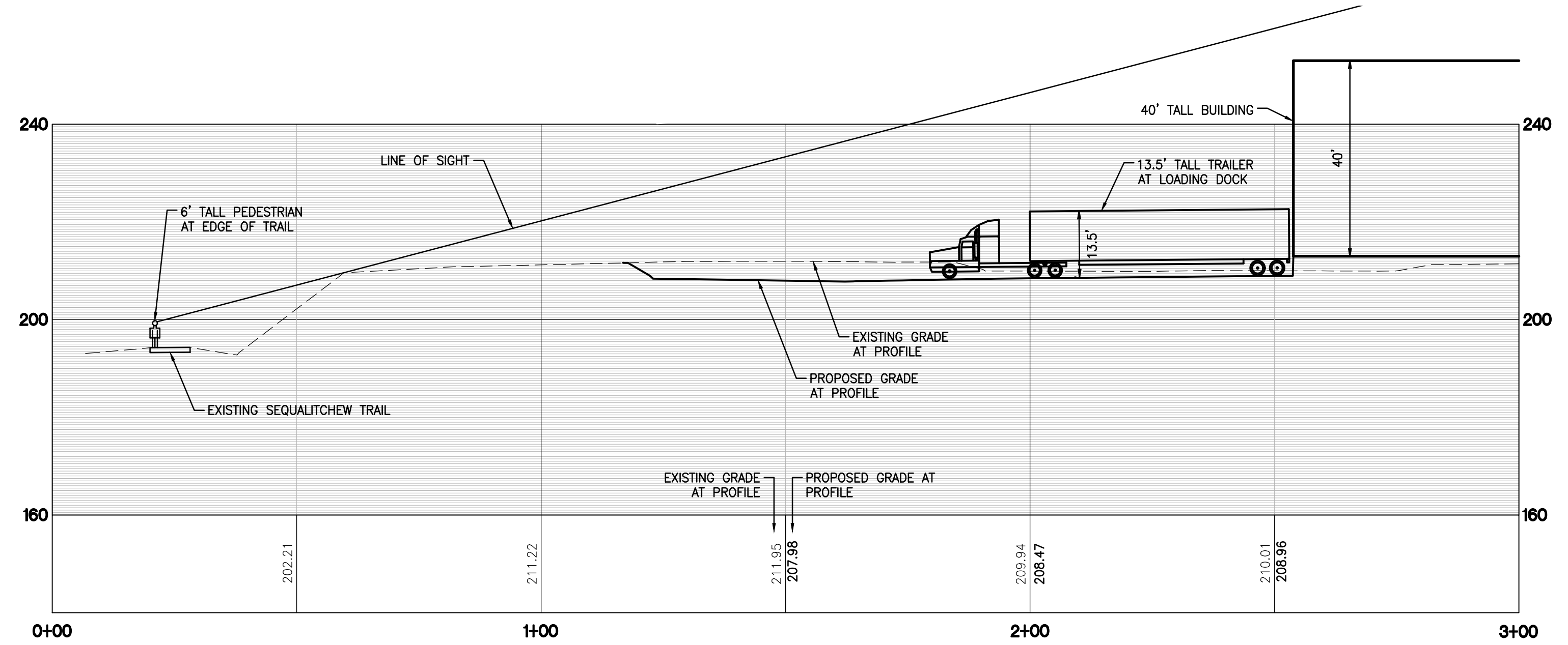
TRAIL LINE OF SIGHT PROFILE B SCALE: HOR: 1" = 20' VERT: 1" = 20'
