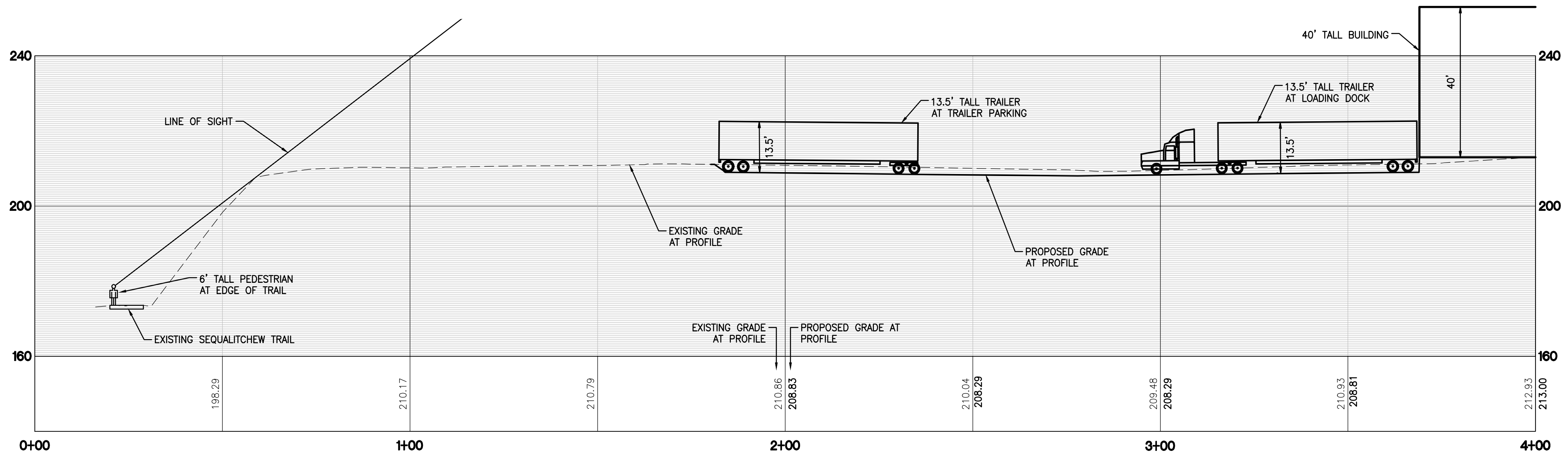
TRAIL LINE OF SIGHT PROFILE A SCALE HOR: 1" = 20' VERT: 1" = 20'
