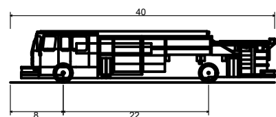
PUMPER FIRE TRUCK PROFILE SCALE: 1" = 20'
