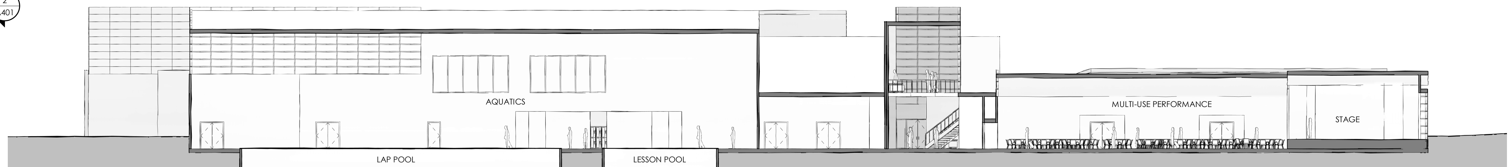
2 SECTION 2 1/16" = 1'-0"
