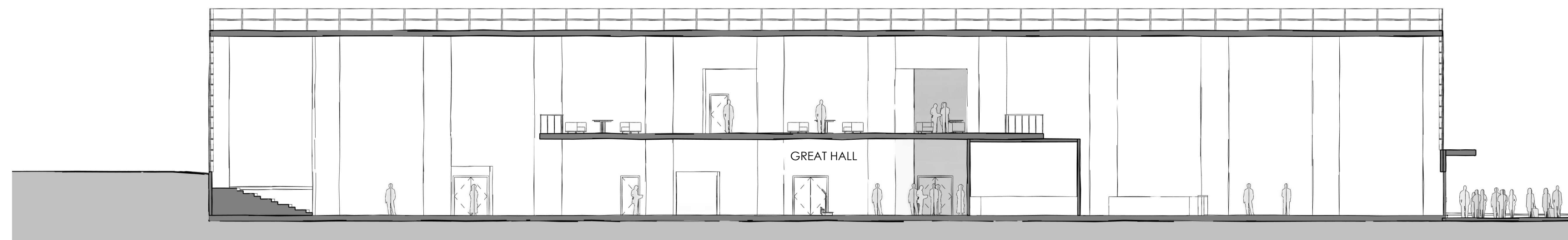
1 SECTION 5 1/16" = 1'-0"
